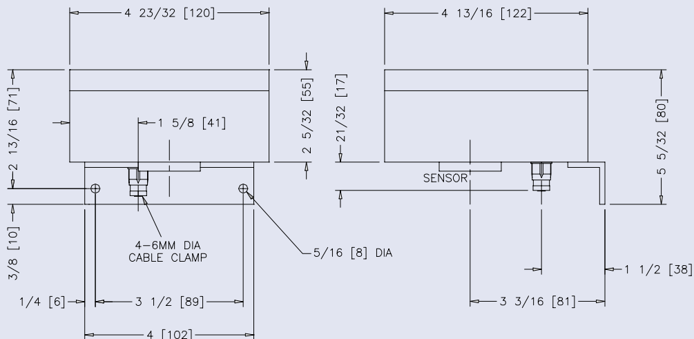
Receiver and Sensor Dimensions (reference only)
