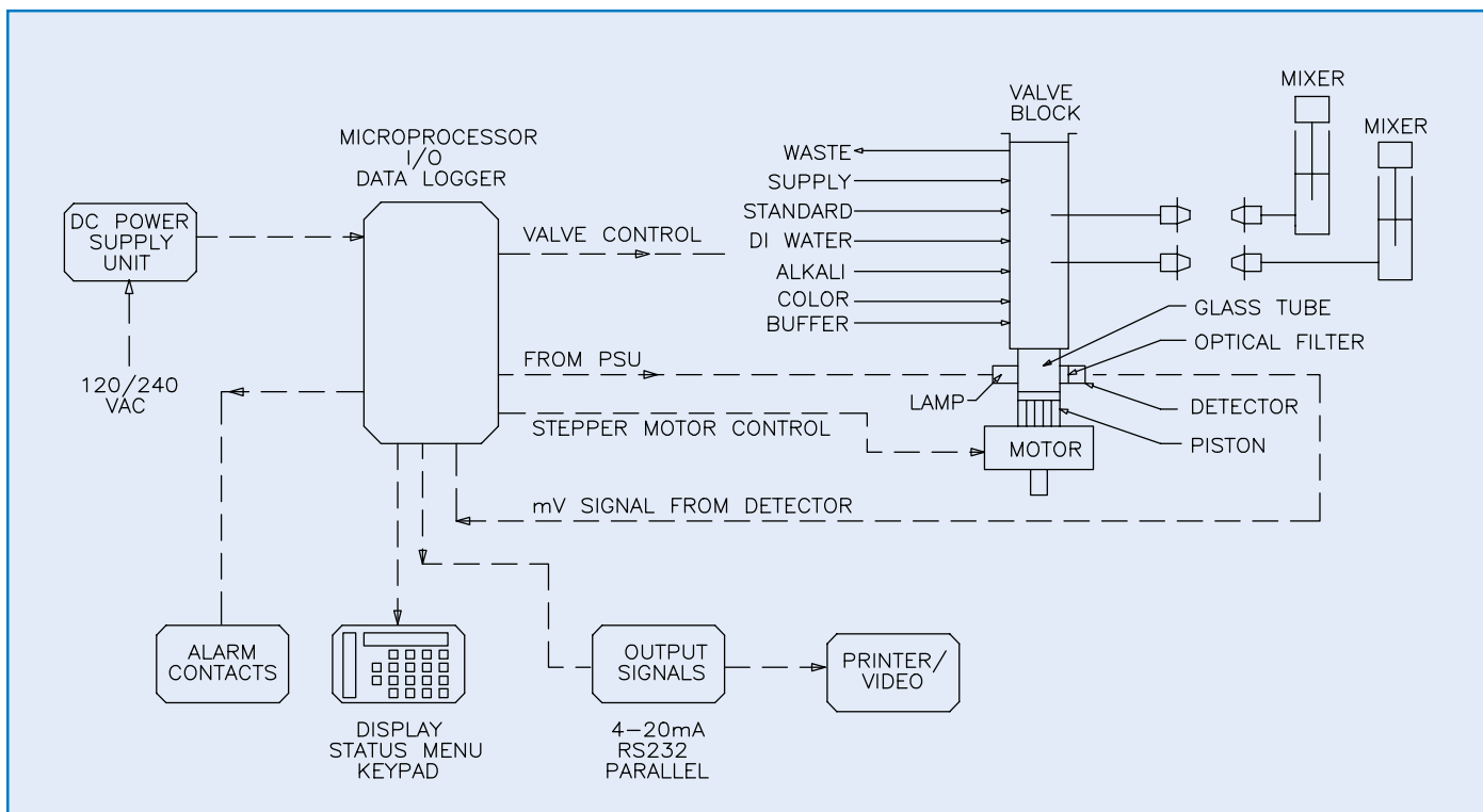
Figure 1 - Manganese Monitor Flow Diagram
