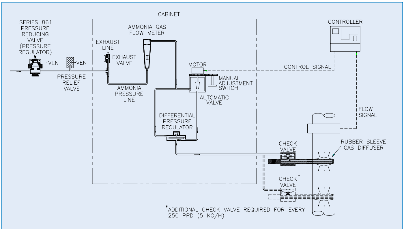
Figure 2 - 1000 PPD (20 kg/h) Maximum Flow Diagram
