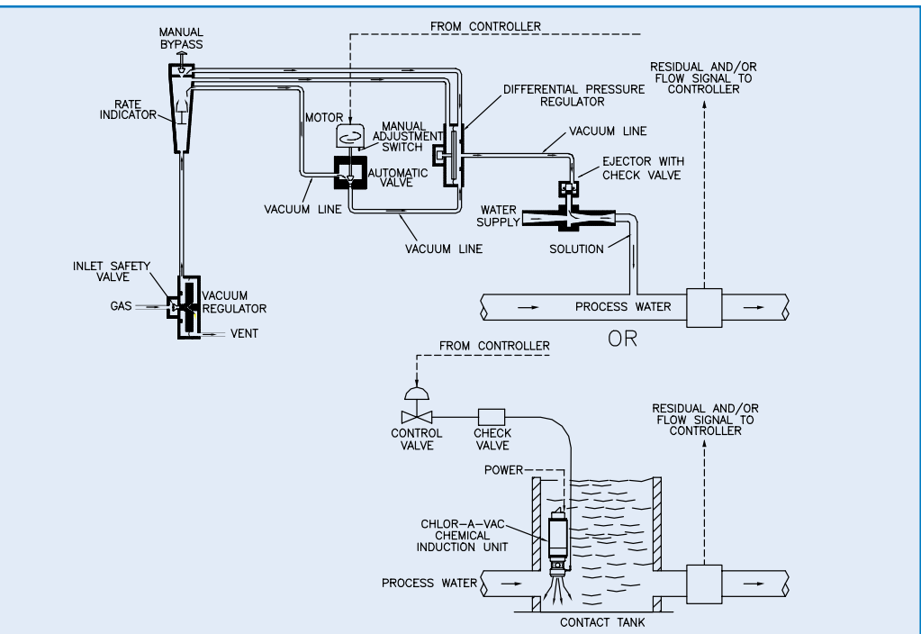
Figure 1 - Automatic Gas Feed System
